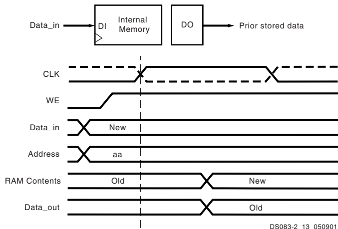
Figure 41: READ_FIRST Mode
