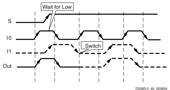
Figure 52: Clock Multiplexer Waveform Diagram
