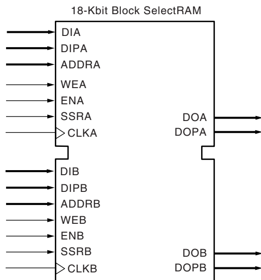
Figure 39: 18 Kb Block SelectRAM+ in Dual-Port Mode
