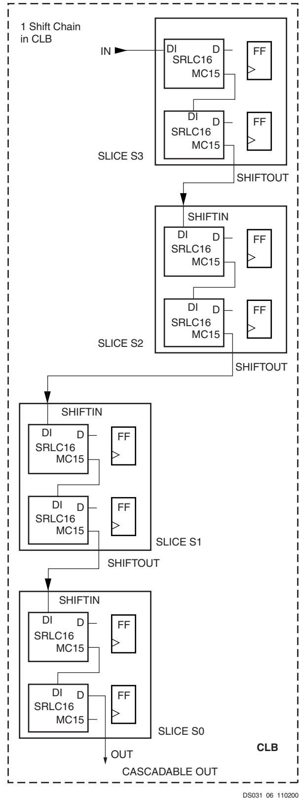
Figure 31: Cascadable Shift Register
